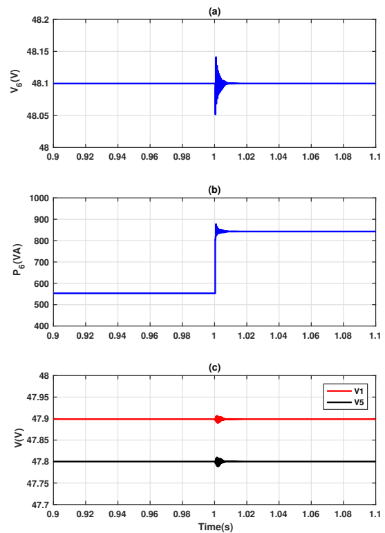
Fig. 9: Dynamic response of DG6 and its neighbors due to a load change at PCC6 at t = 1 s: (a) voltage at PCC6, (b) injected power of DG6, and (c) voltage at PCC1 and PCC5.
