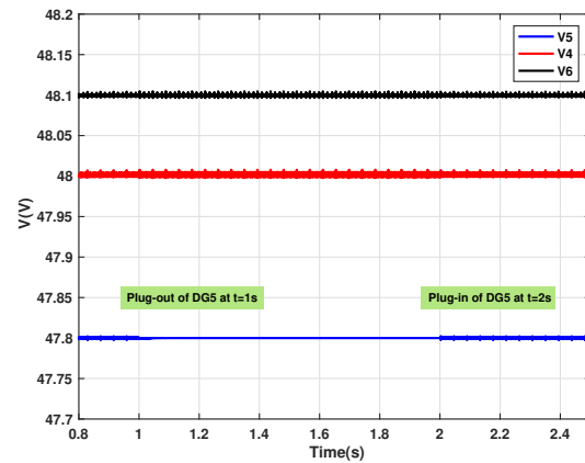
Fig. 11: Performance evaluation of the proposed control strategy under plug-out of DG5 at t = 1s and its plug-in at t = 2s in Case study 6.
