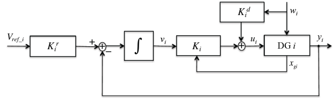
Fig. 3: Block diagram of overall control system of DG i .
