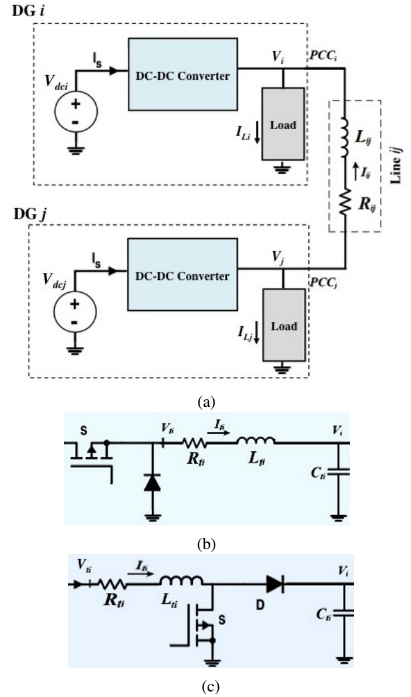
Fig. 2: (a) General configuration of DG i interfaced with a DC-DC converter connected to DG j via the distribution line, (b) model of a buck converter, and (c) model of boost converter.
