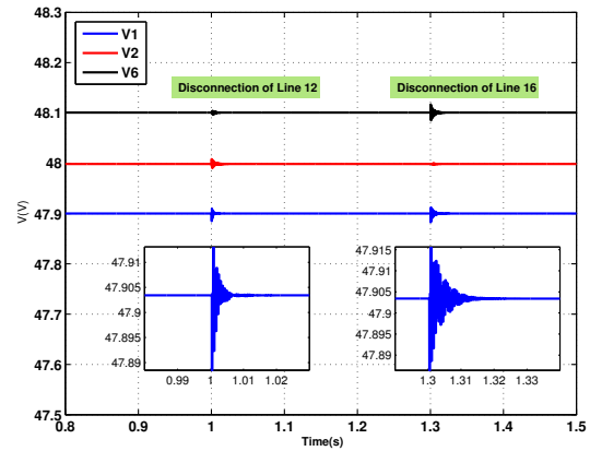
Fig. 8: Dynamic response of DG1, DG2, and DG6 due to changes in microgrid topology at t = 1 s and t = 1.3 s.
