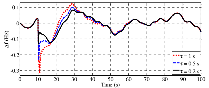
Fig. 7. Impact of communication delay ( \tau ) on the performance of the proposed RDR scheme in response to a 115 MW step load at t=10 s.
