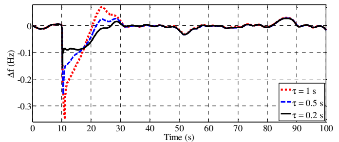
Fig. 8. Performance of the supervisory fuzzy-PI-based coordinator for different RDR delays.
