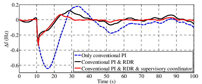
Fig. 9. Performance evaluation of the RDR and supervisory fuzzy-PI-based coordinator in comparison with the conventional PI controller for 1 s communication latency.
