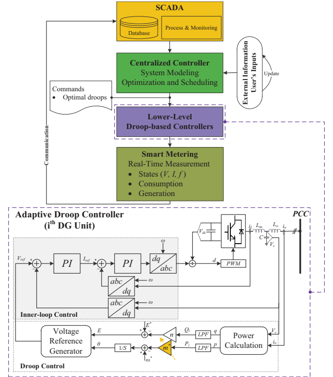
Figure 2. Two-level hybrid control strategy for optimal operation management of DG units
