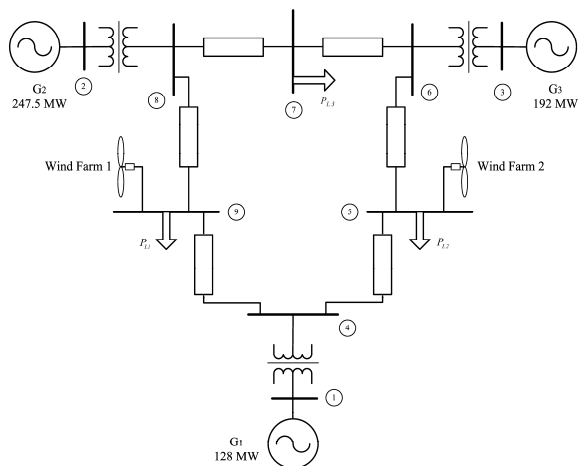
Fig. 1. Single line diagram of the updated nine-bus test system.
