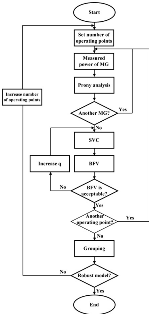
Fig. 2 Flowchart representation of the equivalencing approach
