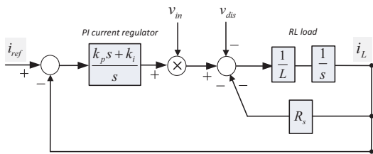
Fig. 4. Block diagram of the current control loop.
