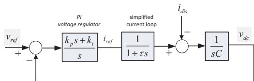
Fig. 5. Block diagram of dc voltage control loop.
