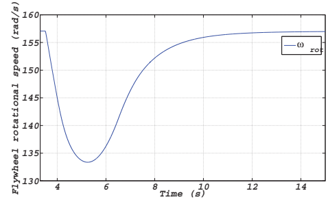
Fig. 6. Flywheel speed propagation throughout the rate limit power strategy transient.
