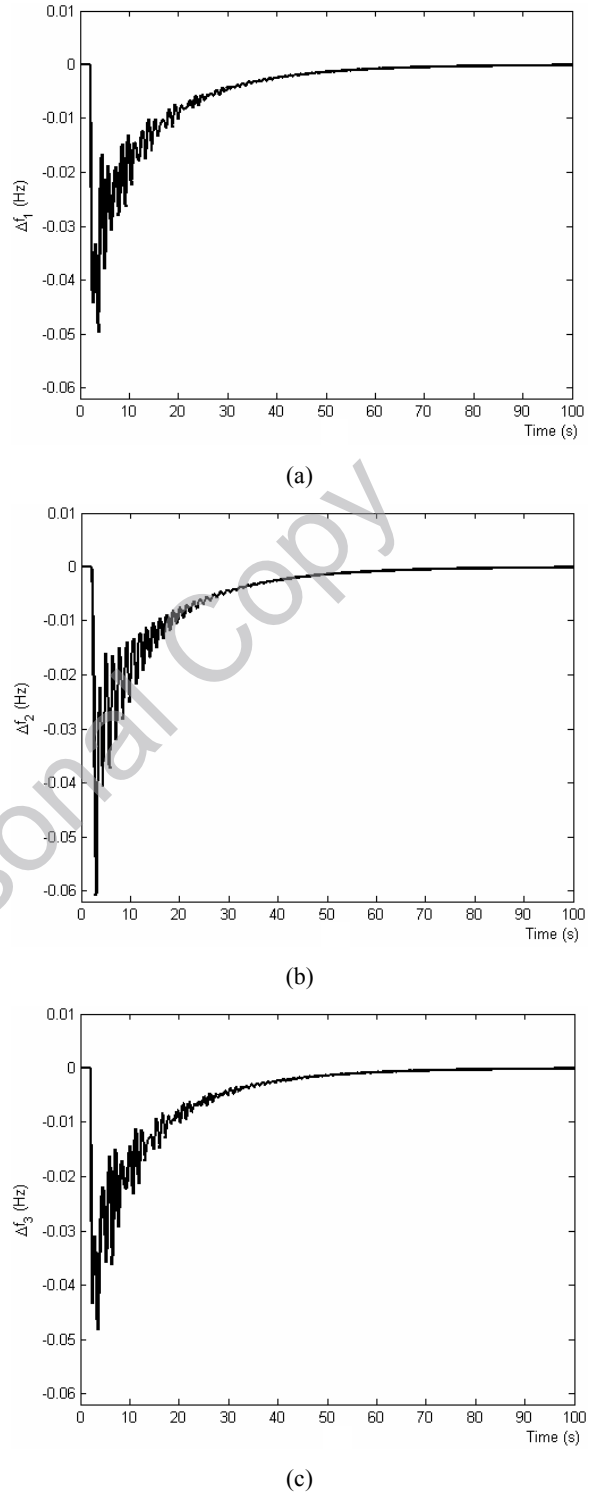
Figure 4 Frequency responses for scenario A, (a) area 1 (b) area 2 (c) area 3
